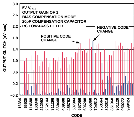
Figure 44. 6 MSB Segment Glitch Energy for +5 V REF
