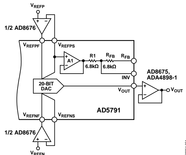
Figure 51. Output Amplifier in Unity-Gain Configuration
