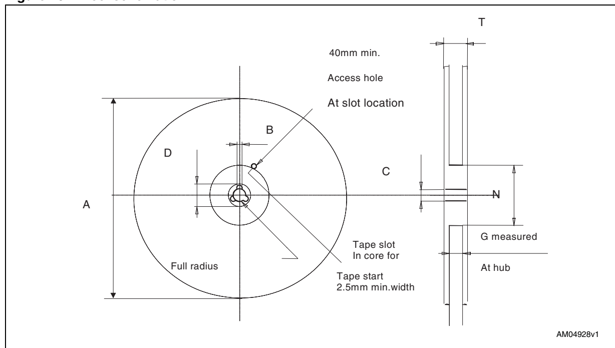
Figure 20. Reel schematic
