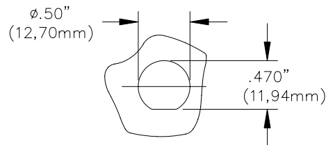
PANEL CUTOUT
