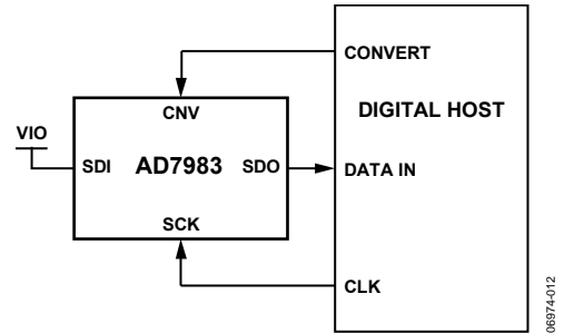
Figure 26. \overline{\text{CS}} Mode, 3-Wire Without Busy Indicator Connection Diagram (SDI High)
