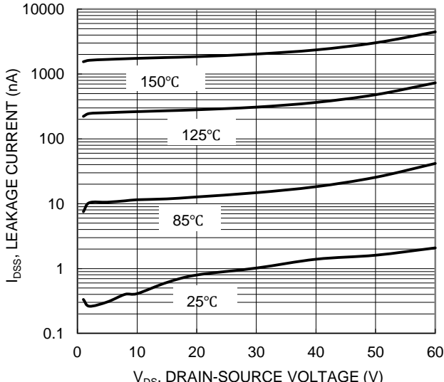
Figure 9. Typical Drain-Source Leakage Current vs. Voltage
