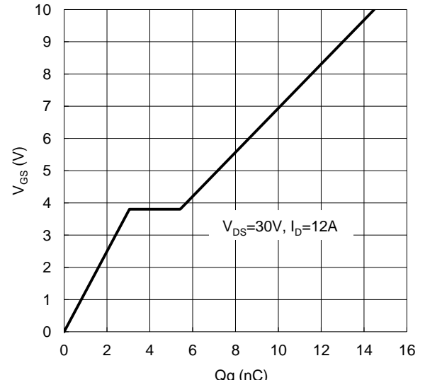
Figure 10. Gate Charge
