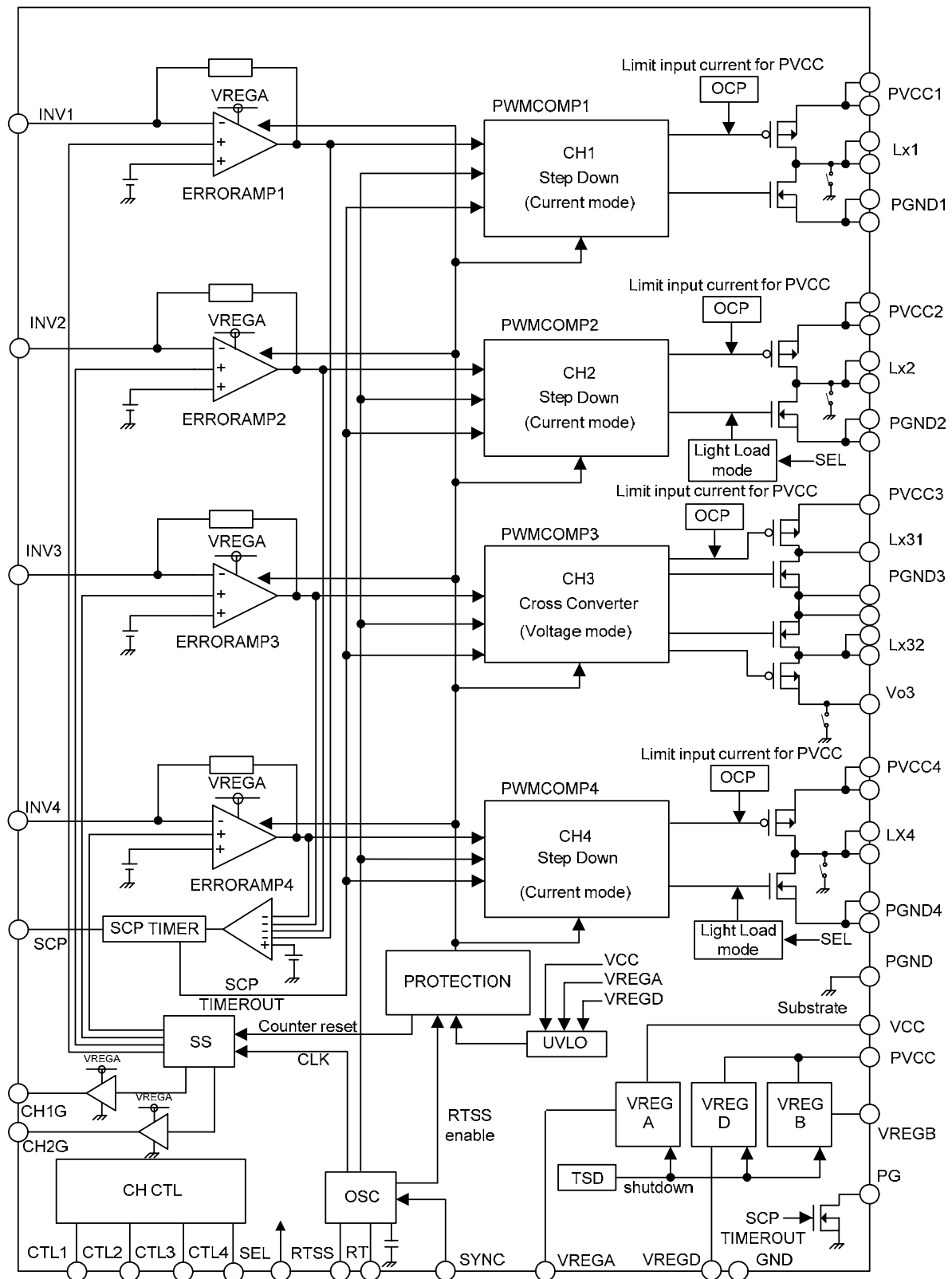
Figure. 3 block diagram
