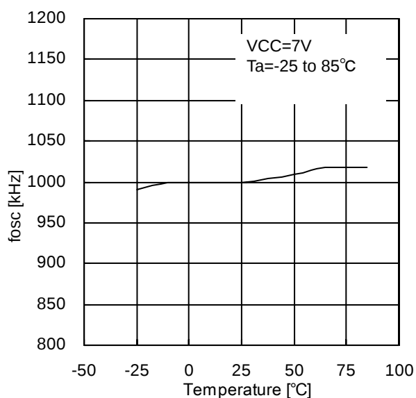
Figure.25 fosc - Ta
