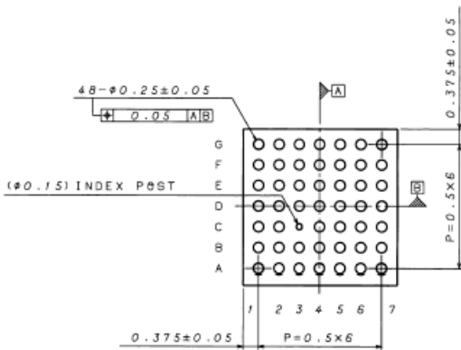
Figure. 64 Package dimensions
