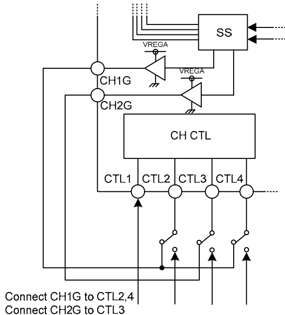
Figure.56 example of startup sequence control
