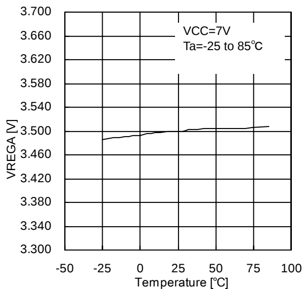
Figure.15 VREGA – Ta
