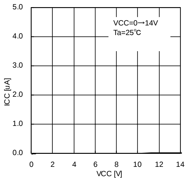
Figure.10 ICC (OFF) - VCC
