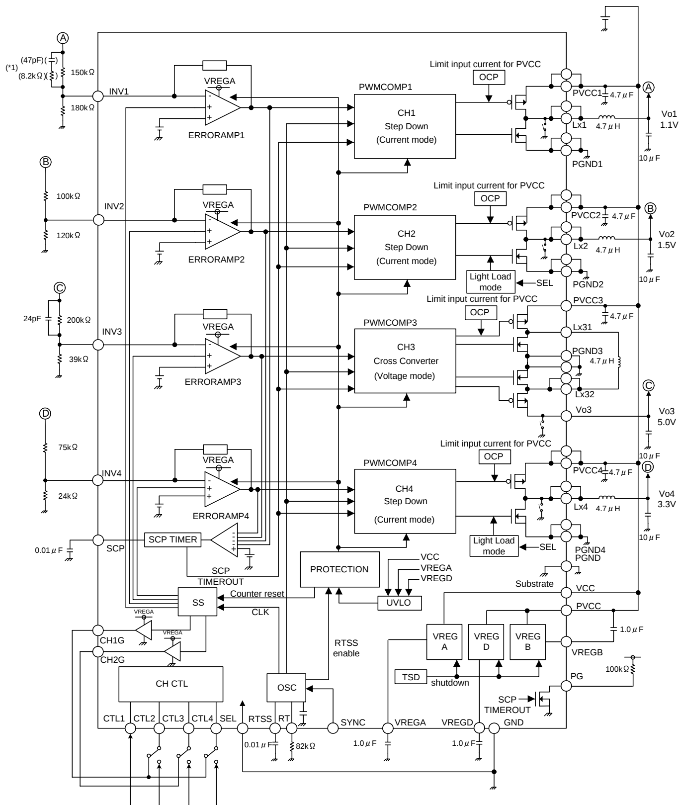
Figure. 4 Application circuit 1
