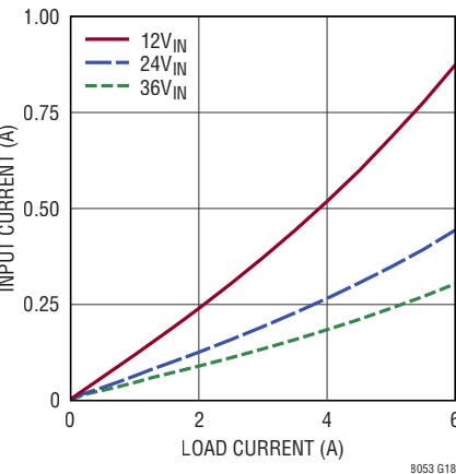
LTM8053 Input vs Load Current, V_{OUT} = 1.2\text{V} , BIAS = 5V
