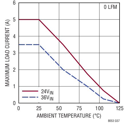
LTM8053 Derating, V_{OUT} = -3.3V , BIAS Tied to LTM8053 GND, DC1934A Demo Board
