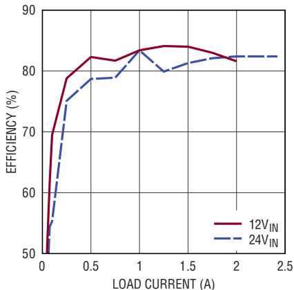
LTM8053 Efficiency vs Load Current, V_{OUT} = -15\text{V} , BIAS Tied to LTM8053 GND
