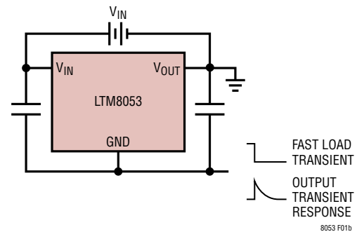
Figure 1b. Any Output Voltage Transient Appears on LTM8053/LTM8053-1 GND
