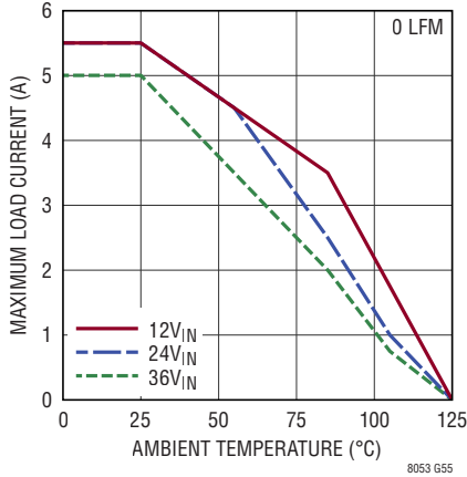
LTM8053 Derating, V_{OUT} = 5V , BIAS = 5V, DC1934A Demo Board
