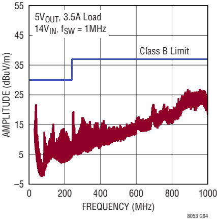
LTM8053 CISPR32 Class B Emissions DC1934A Demo Board, No EMI Filter ( C_{10} = 0.1\mu\text{F} , Short L1, Open C7)
