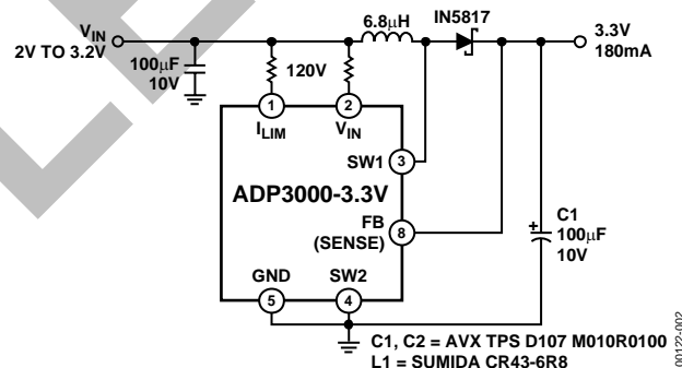
Figure 2. Typical Application
