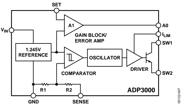
Figure 8. Functional Block Diagram for Fixed Version
