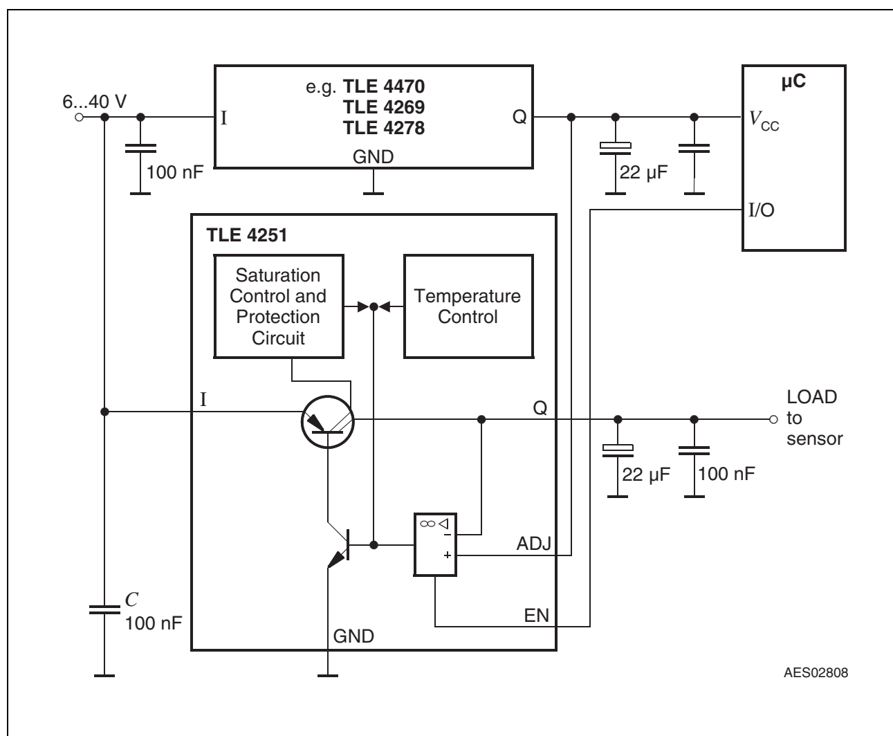
Figure 3 Application Circuit
