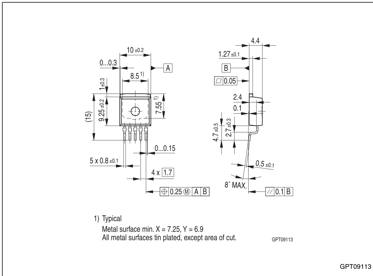
Figure 5 PG-TO263-5-1 (Plastic Transistor Single Outline)
