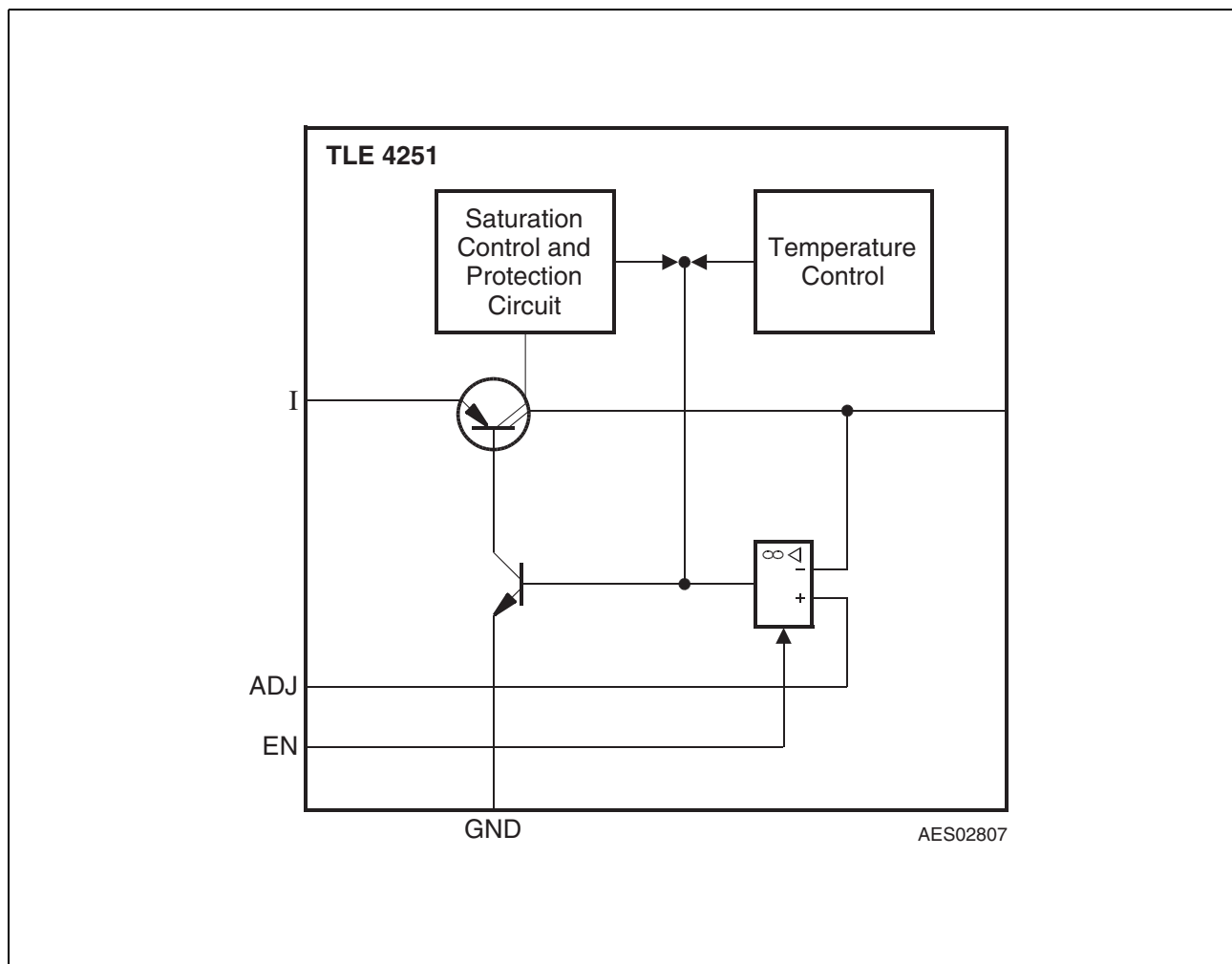
Figure 2 Block Diagram
