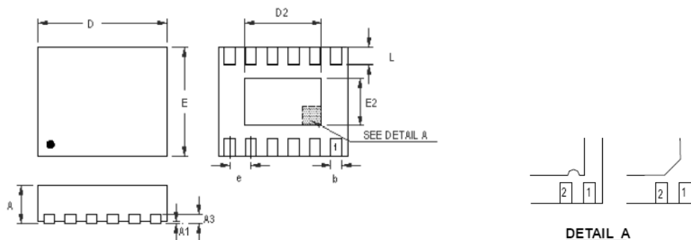
DETAIL A
