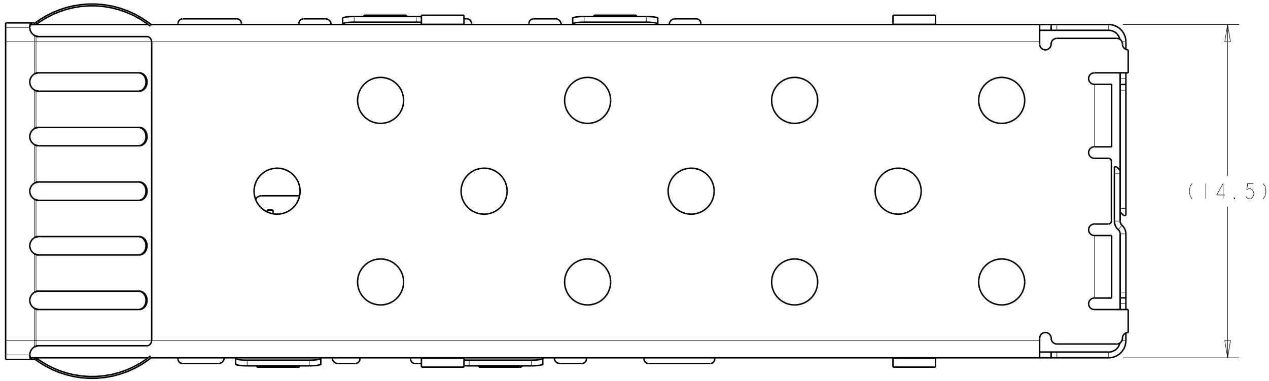
2007215-1 TOP VIEW
