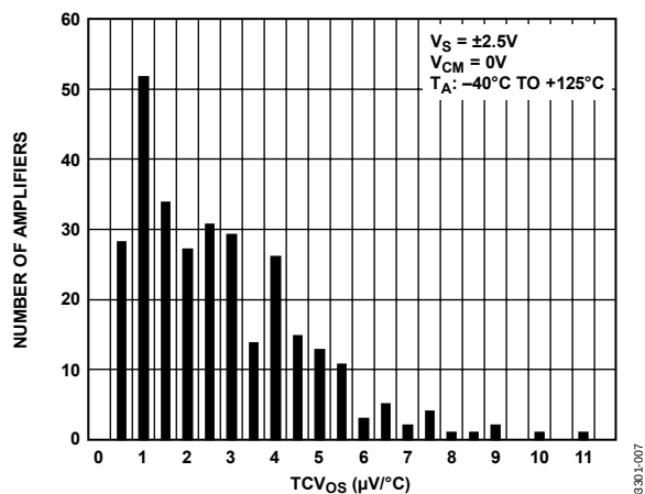
Figure 7. TCV_{OS} Distribution
