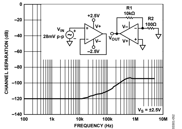
Figure 52. Channel Separation vs. Frequency.
