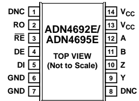
Figure 4. ADN4692E/ADN4695E Pin Configuration
