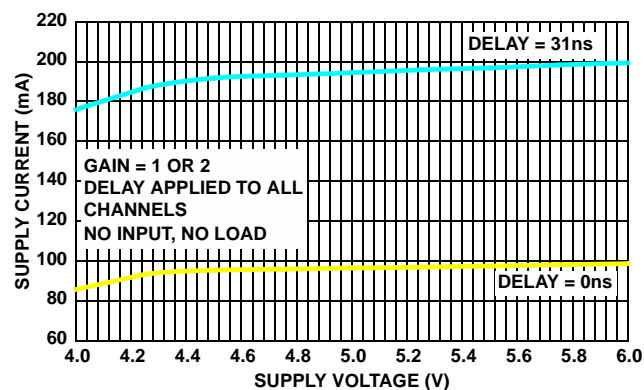
FIGURE 29. ISL59922 I_{SUPPLY+} vs V_{SUPPLY+}
