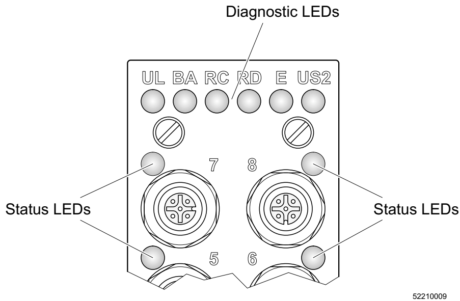
Figure 8: Arrangement of LEDs
