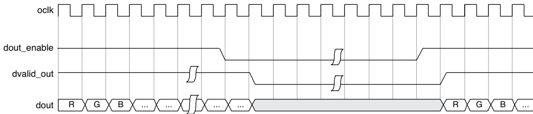
Figure 2-7. dout_enable Control Timing
