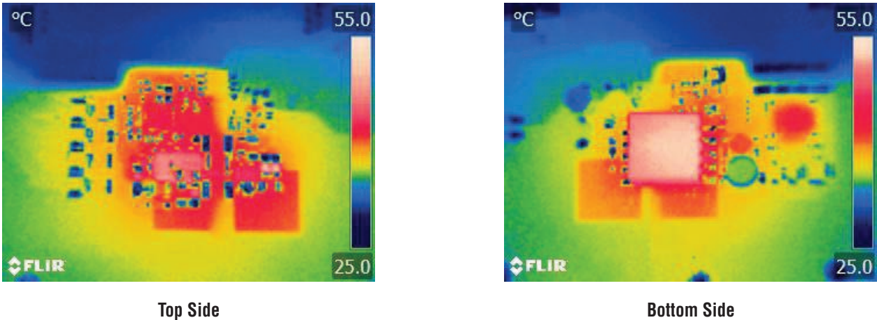
Figure 1. Thermal Pictures – V_{PORT} = 57V, 12V/1.9A
