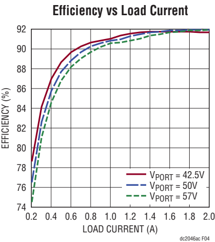
Figure 2. Efficiency (End to End)
