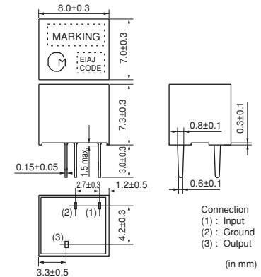
SFPLA Series
