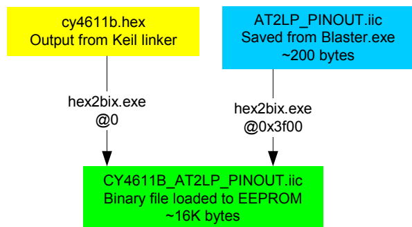
Figure 4: Output files
