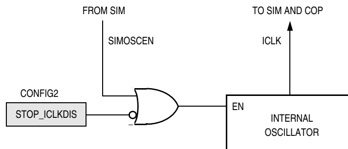
Figure 5-4. Internal Oscillator
