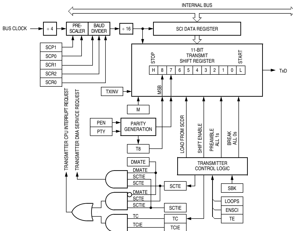
Figure 7-4. SCI Transmitter
