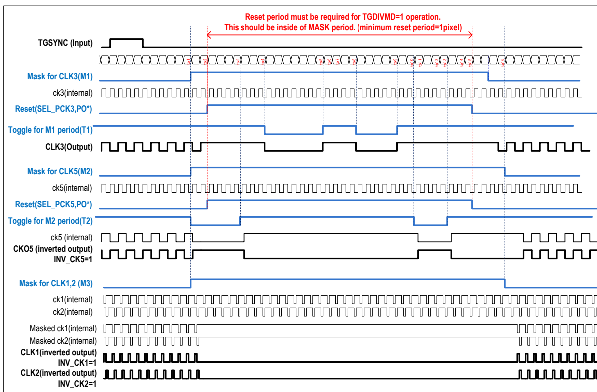
Figure 27 TG Divide Mode
