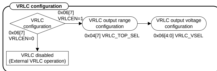
Figure 44 VRCL Configuration
