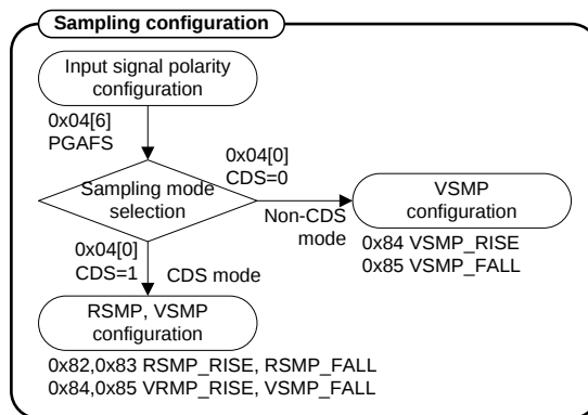
Figure 42 Sampling Configuration
