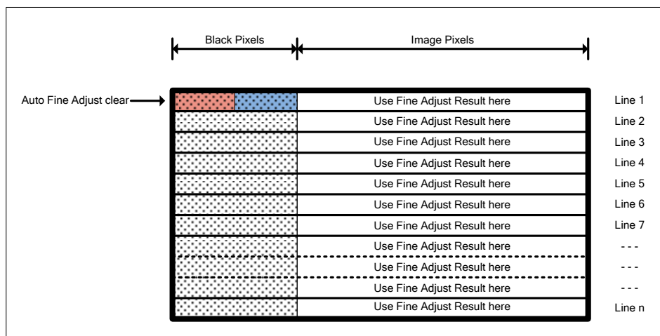
Figure 31 Scenario 2
