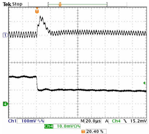
Fig-3.3V-7: Output voltage response for V_{out}=3.3V to negative load current step-change from 10A to 5A with slew rate of -5A/\mu s at V_{in}=5.0V . C_o=47\mu F \times 2 ceramic. Top trace: output voltage (100mV/div.) Bottom trace: load current (5A/div.) Time scale: 20μs/div.
