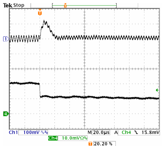
Fig-1.5V-7: Output voltage response for V_{out}=1.5V to positive load current step-change from 10A to 5A with slew rate of -5A/\mu s at V_{in}=5.0V . C_o=47\mu F \times 2 ceramic. Top trace: output voltage (100mV/div.) Bottom trace: load current (5A/div.) Time scale: 20μs/div.
