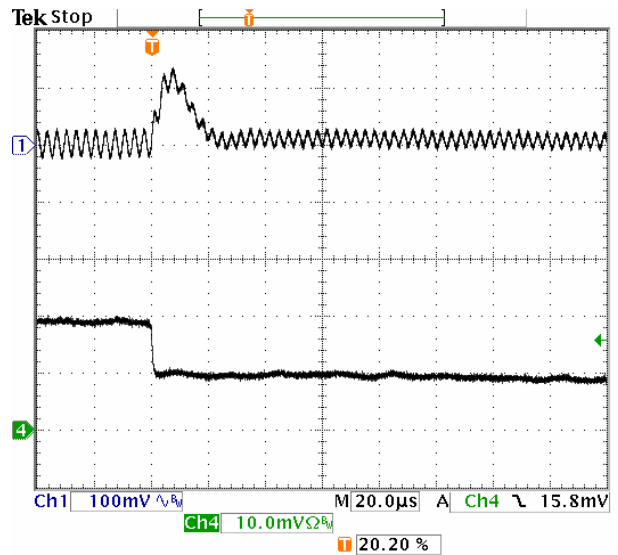
Fig-2.0V-7: Output voltage response for V_{out}=2.0V to positive load current step-change from 10A to 5A with slew rate of -5A/\mu s at V_{in}=5.0V . C_o=47\mu F \times 2 ceramic. Top trace: output voltage (100mV/div.) Bottom trace: load current (5A/div.) Time scale: 20μs/div.
