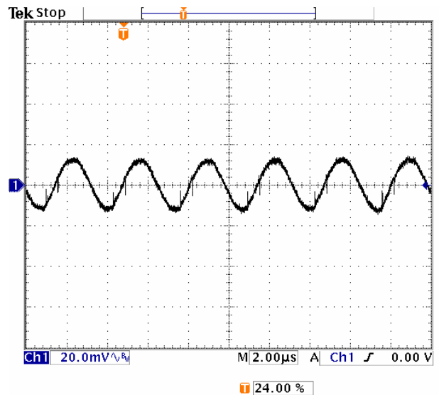
Fig-0.7255V-5: Output voltage ripple (20mV/div.) for V_{out}=0.7525V at full rated load current into a resistive load with external capacitance 47\mu F \times 2 ceramic + 1\mu F ceramic at V_{in}=5.0V . Time scale: 2μs/div
