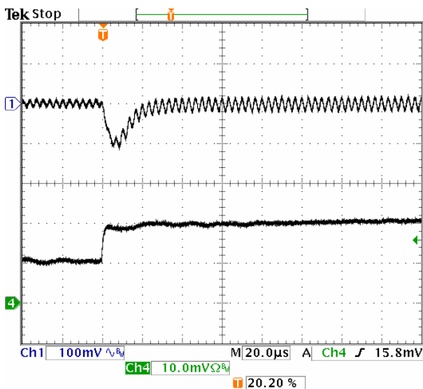
Fig-1.0V-6: Output voltage response for V_{out}=1.0V to positive load current step-change from 5A to 10A with slew rate of 5A/\mu s at V_{in}=5.0V . C_o=47\mu F \times 2 ceramic. Top trace: output voltage (100mV/div.) Bottom trace: load current (5A/div.) Time scale: 20μs/div.
