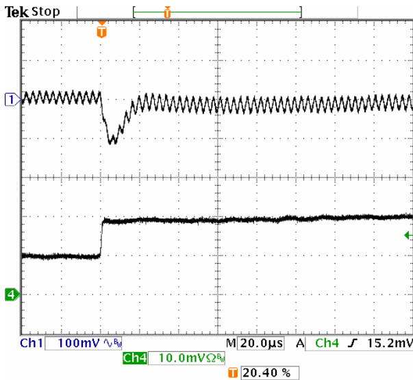
Fig-3.3V-6: Output voltage response for V_{out}=3.3V to positive load current step-change from 5A to 10A with slew rate of 5A/\mu s at V_{in}=5.0V . C_o=47\mu F \times 2 ceramic. Top trace: output voltage (100mV/div.) Bottom trace: load current (5A/div.) Time scale: 20μs/div.
