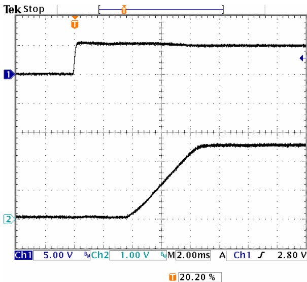
Fig-2.5V-4: Turn-on transient for V_{out}=2.5V with application of V_{in} at full rated load current (resistive) and 47\mu F \times 2 external capacitance at V_{in}=5.0V . Top trace: V_{in} (5V/div.) Bottom trace: output voltage (1V/div.) Time scale: 2ms/div.
