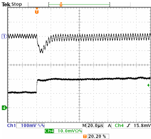
Fig-1.8V-6: Output voltage response for V_{out}=1.8V to positive load current step-change from 5A to 10A with slew rate of 5A/\mu s at V_{in}=5.0V . C_o=47\mu F \times 2 ceramic. Top trace: output voltage (100mV/div.) Bottom trace: load current (5A/div.) Time scale: 20μs/div.
