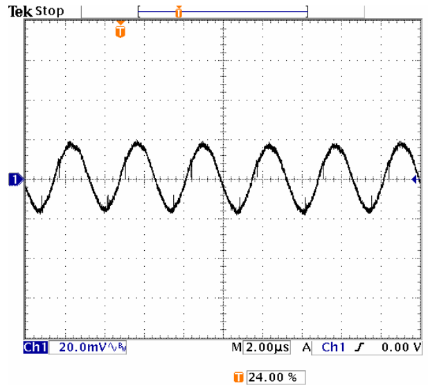
Fig-1.2V-5: Output voltage ripple (20mV/div.) for V_{out}=1.2V at full rated load current into a resistive load with external capacitance 47\mu F \times 2 ceramic + 1\mu F ceramic at V_{in}=5.0V . Time scale: 2μs/div
