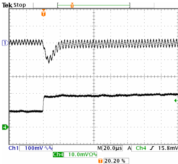
Fig-2.0V-6: Output voltage response for V_{out}=2.0V to positive load current step-change from 5A to 10A with slew rate of 5A/\mu s at V_{in}=5.0V . C_o=47\mu F \times 2 ceramic. Top trace: output voltage (100mV/div.) Bottom trace: load current (5A/div.) Time scale: 20μs/div.
