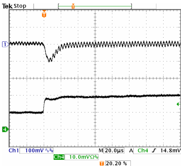
Fig-0.7525V-6: Output voltage response for V_{out}=0.7525V to positive load current step-change from 5A to 10A with slew rate of 5A/\mu s at V_{in}=5.0V . C_o=47\mu F \times 2 ceramic. Top trace: output voltage (100mV/div.) Bottom trace: load current (5A/div.) Time scale: 20μs/div.
