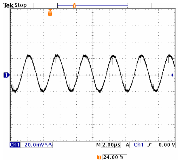
Fig-2.5V-5: Output voltage ripple (20mV/div.) for V_{out}=2.5V at full rated load current into a resistive load with external capacitance 47\mu F \times 2 ceramic + 1\mu F ceramic at V_{in}=5.0V . Time scale: 2μs/div
