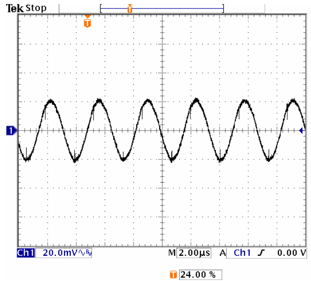
Fig-1.8V-5: Output voltage ripple (20mV/div.) for V_{out}=1.8V at full rated load current into a resistive load with external capacitance 47\mu F \times 2 ceramic + 1\mu F ceramic at V_{in}=5.0V . Time scale: 2μs/div
