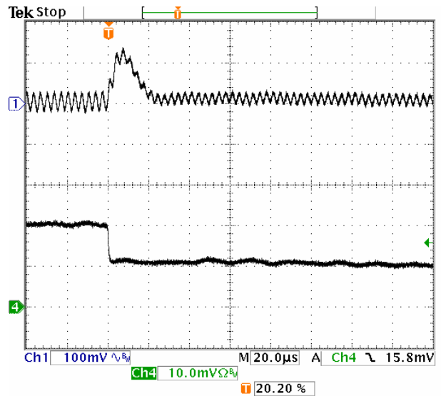
Fig-1.8V-7: Output voltage response for V_{out}=1.8V to positive load current step-change from 10A to 5A with slew rate of -5A/\mu s at V_{in}=5.0V . C_o=47\mu F \times 2 ceramic. Top trace: output voltage (100mV/div.) Bottom trace: load current (5A/div.) Time scale: 20μs/div.
