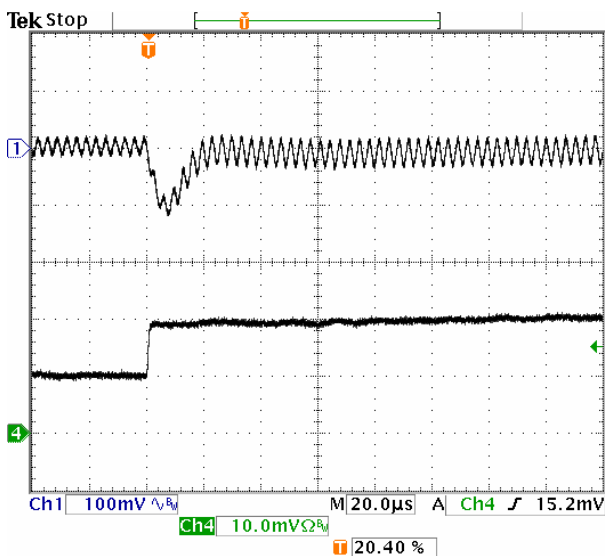
Fig-2.5V-6: Output voltage response for V_{out}=2.5V to positive load current step-change from 5A to 10A with slew rate of 5A/\mu s at V_{in}=5.0V . C_o=47\mu F \times 2 ceramic. Top trace: output voltage (100mV/div.) Bottom trace: load current (5A/div.) Time scale: 20μs/div.
