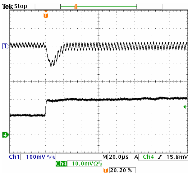
Fig-1.5V-6: Output voltage response for V_{out}=1.5V to positive load current step-change from 5A to 10A with slew rate of 5A/\mu s at V_{in}=5.0V . C_o=47\mu F \times 2 ceramic. Top trace: output voltage (100mV/div.) Bottom trace: load current (5A/div.) Time scale: 20μs/div.
