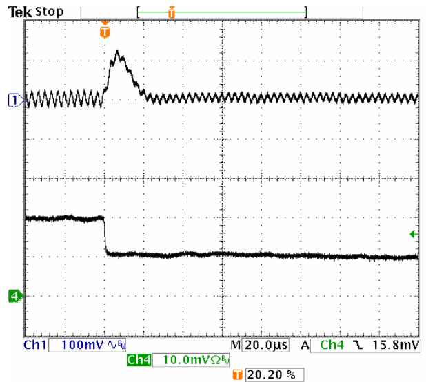
Fig-1.2V-7: Output voltage response for V_{out}=1.2V to positive load current step-change from 10A to 5A with slew rate of -5A/\mu s at V_{in}=5.0V . C_o=47\mu F \times 2 ceramic. Top trace: output voltage (100mV/div.) Bottom trace: load current (5A/div.) Time scale: 20μs/div.
