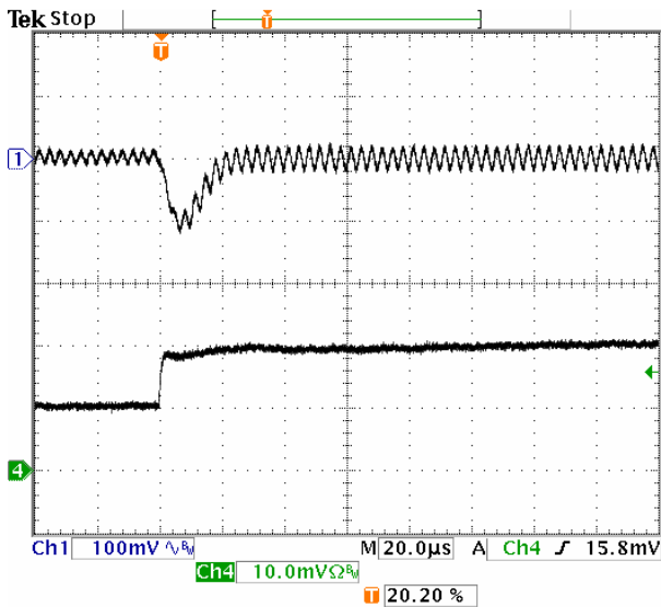
Fig-1.2V-6: Output voltage response for V_{out}=1.2V to positive load current step-change from 5A to 10A with slew rate of 5A/\mu s at V_{in}=5.0V . C_o=47\mu F \times 2 ceramic. Top trace: output voltage (100mV/div.) Bottom trace: load current (5A/div.) Time scale: 20μs/div.
