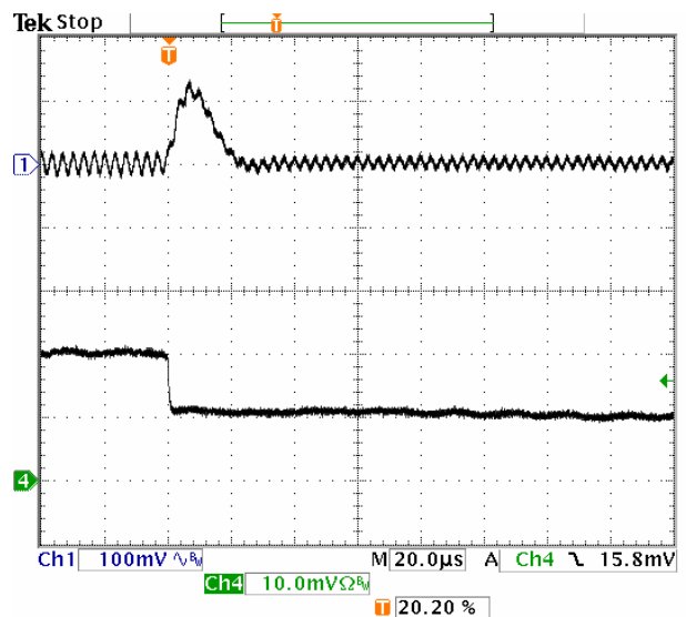
Fig-1.0V-7: Output voltage response for V_{out}=1.0V to positive load current step-change from 10A to 5A with slew rate of -5A/\mu s at V_{in}=5.0V . C_o=47\mu F \times 2 ceramic. Top trace: output voltage (100mV/div.) Bottom trace: load current (5A/div.) Time scale: 20μs/div.
