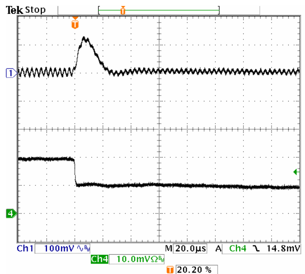
Fig-0.7525V-7: Output voltage response for V_{out}=0.7525V to positive load current step-change from 10A to 5A with slew rate of -5A/\mu s at V_{in}=5.0V . C_o=47\mu F \times 2 ceramic. Top trace: output voltage (100mV/div.) Bottom trace: load current (5A/div.) Time scale: 20μs/div.
