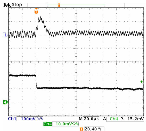
Fig-2.5V-7: Output voltage response for V_{out}=2.5V to positive load current step-change from 10A to 5A with slew rate of -5A/\mu s at V_{in}=5.0V . C_o=47\mu F \times 2 ceramic. Top trace: output voltage (100mV/div.) Bottom trace: load current (5A/div.) Time scale: 20μs/div.
