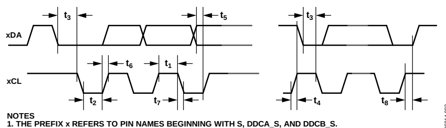
Figure 2. I²C Timing
