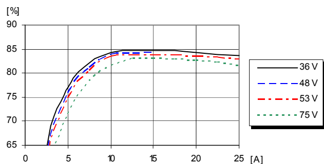
Efficiency vs. load current and input voltage at T_{P1} = +25^{\circ}\text{C}
