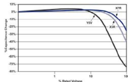
Figure 8 - Typical Variation of Capacitance with Applied DC Voltage tion factor change.)
