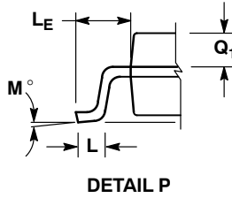
DETAIL P
