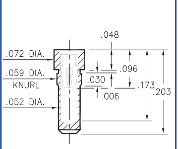
0676-0-15-XX-30-XX-10-0 Press-fit in .057 mounting hole
