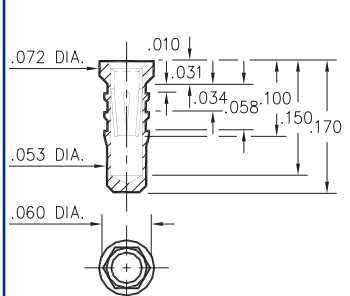
0252-0-15-XX-32-XX-10-0 Hex press-fit in .057 plated thru hole
