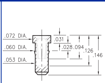
0668-0-15-XX-30-XX-10-0 Press-fit in .057 mounting hole
