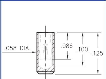
0673-0-15-XX-30-XX-10-0 Surface Mount
