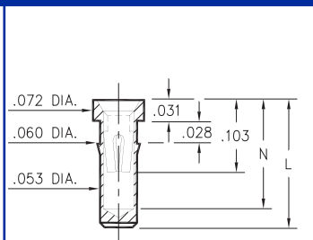
XXX3-0-15-XX-30-XX-10-0 Press-fit in .057 mounting hole
