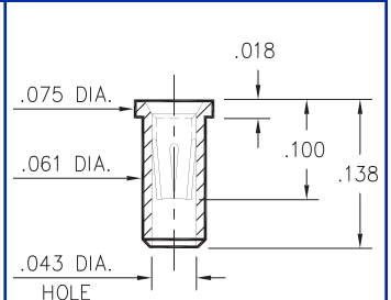
0666-0-15-XX-32-XX-10-0 Solder mount in .064 min. mounting hole Also available on 24mm wide carrier tape: 1,500 parts per 13" reel. Order as: 0666-0-57-XX-32-XX-10-0
