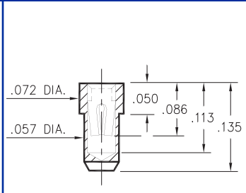
0670-0-15-XX-30-XX-10-0 Solder mount in .060 min. mounting hole
