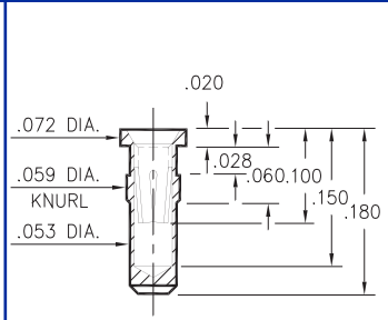
0678-0-15-XX-32-XX-10-0 Press-fit in .057 mounting hole
