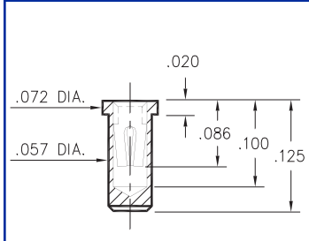
0669-0-15-XX-30-XX-10-0 Solder mount in .060 min. mounting hole Also available on 16mm wide carrier tape: 1,700 parts per 13" reel. Order as: 0669-0-57-XX-30-XX-10-0
