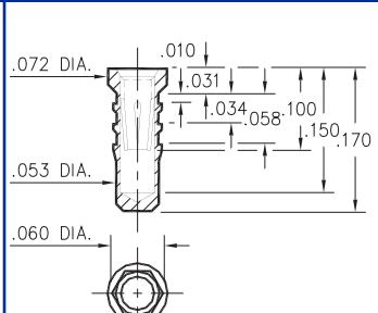
0252-0-15-XX-32-XX-10-0 Hex press-fit in .057 plated thru hole
