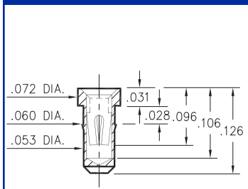
0341-0-15-XX-30-XX-10-0 Solder mount in .073 mounting hole Also available on 12mm wide carrier tape: 1,400 parts per 13" reel. Order as: 0341-0-57-XX-30-XX-10-0
