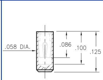
0673-0-15-XX-30-XX-10-0 Surface Mount
