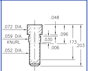
0676-0-15-XX-30-XX-10-0 Press-fit in .057 mounting hole
