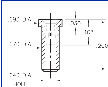
0341-0-15-XX-30-XX-10-0 Solder mount in .073 mounting hole Also available on 12mm wide carrier tape: 1,400 parts per 13" reel. Order as: 0341-0-57-XX-30-XX-10-0
