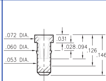
0668-0-15-XX-30-XX-10-0 Press-fit in .057 mounting hole
