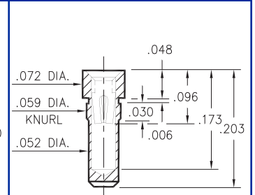
0676-0-15-XX-30-XX-10-0 Press-fit in .057 mounting hole
