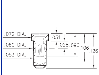
0697-0-15-XX-30-XX-10-0 Press-fit in .057 mounting hole
