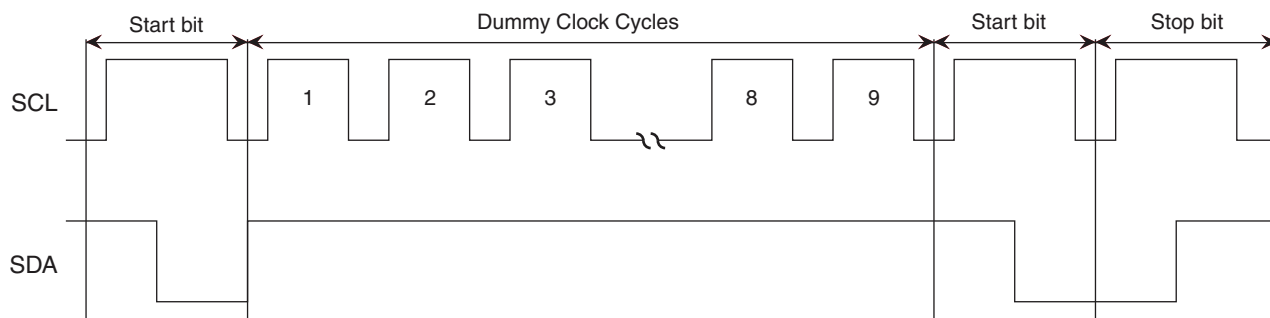
Figure 4-1. Software Reset
