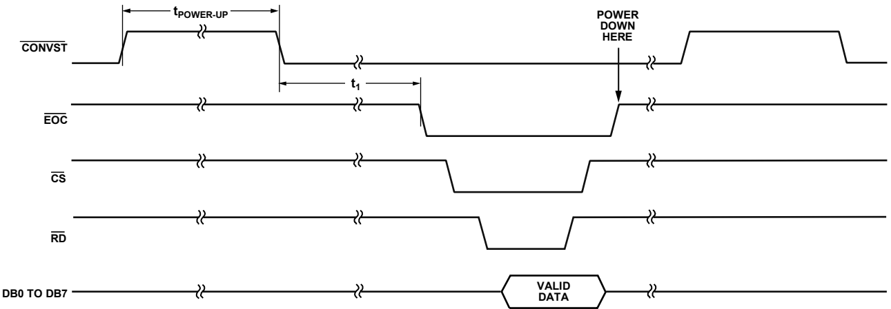
Figure 22. Mode 2 Operation
