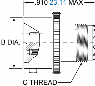
2M803-004-01
