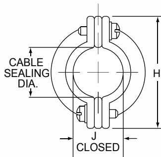
SADDLE CLAMP
