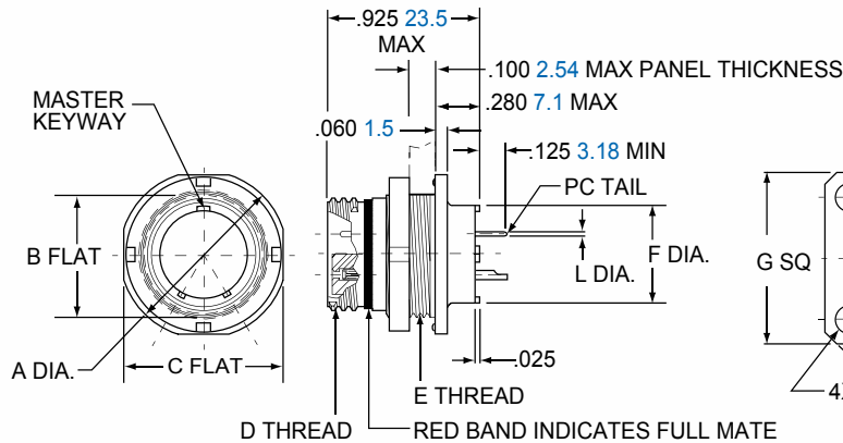
2M801-011-07 2M801-033-07
