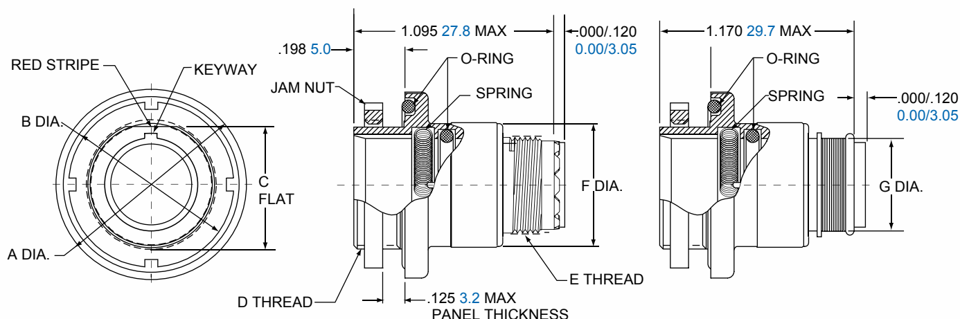
2M804-004-07
