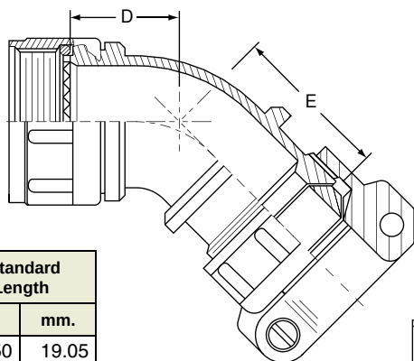
45° ENTRY ROTATABLE COUPLING 2M380MB137
