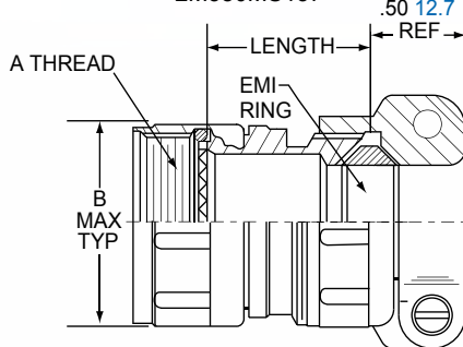
STRAIGHT ENTRY ROTATABLE COUPLING 2M380MS137
