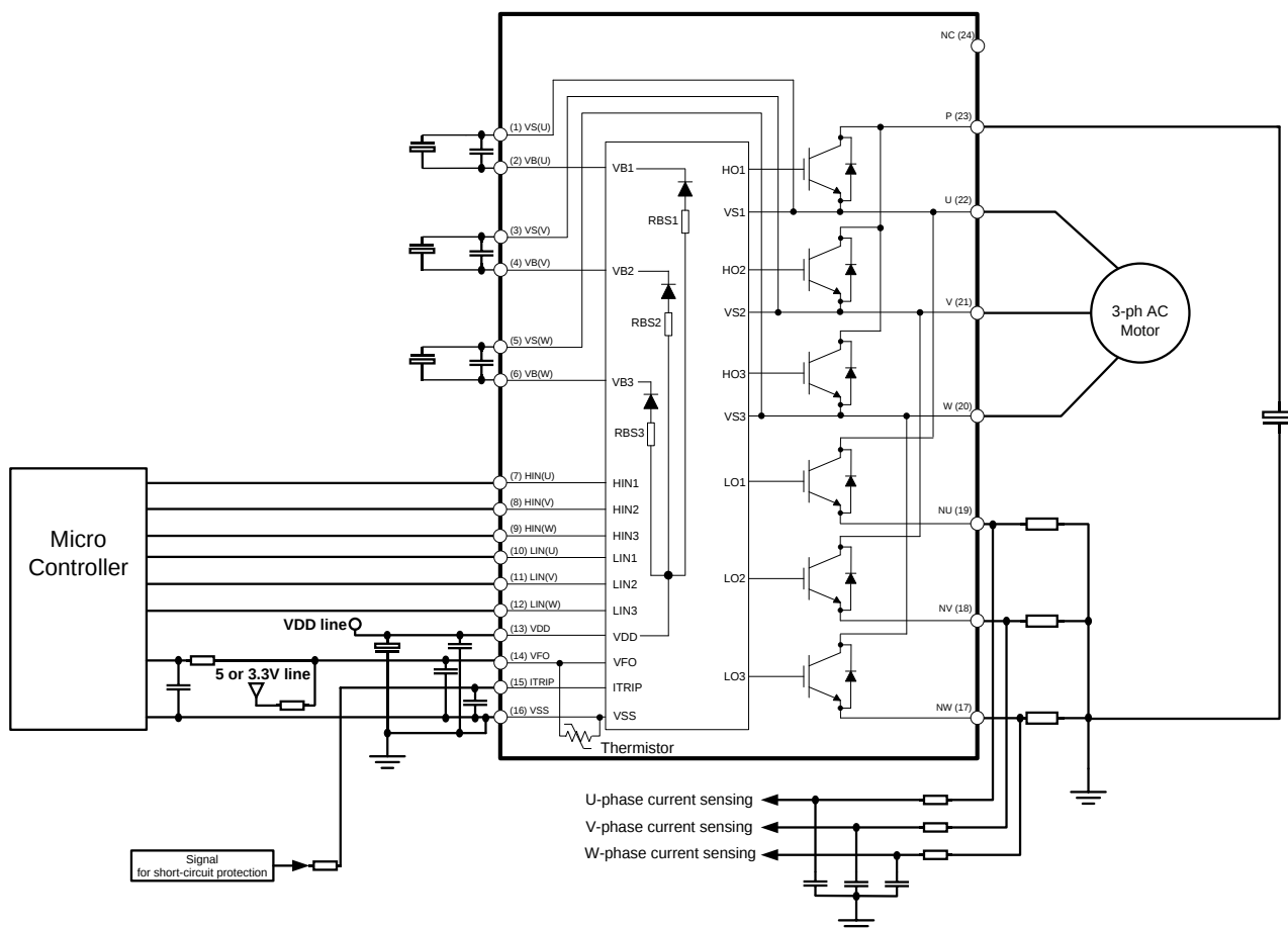
Figure 9: Application circuit
