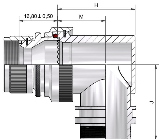
90° BACKSHELL - TYPE 2
