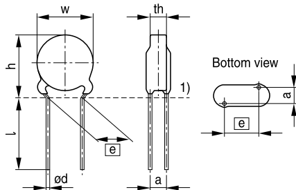
1) Seating plane to IEC 60717
