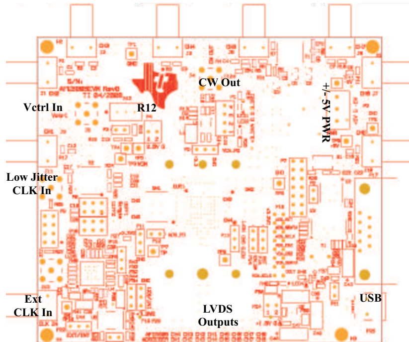
Figure 2. AFE5804EVM I/O Connectors and Locations
