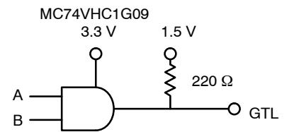
Figure 9. GTL Driver
