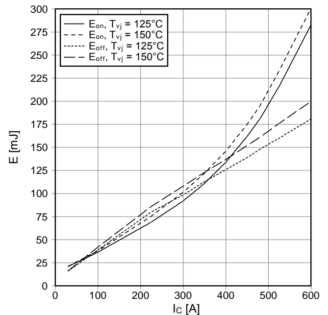
Schaltverluste IGBT-Wechselr. (typisch) switching losses IGBT-inverter (typical) E_{on} = f(I_C), E_{off} = f(I_C) V_{GE} = \pm 15\text{ V}, R_{Gon} = 3.3\ \Omega, R_{Goff} = 4.7\ \Omega, V_{CE} = 900\text{ V}
