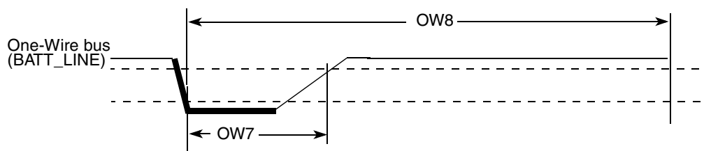
Figure 44. Write 1 Sequence Timing Diagram
