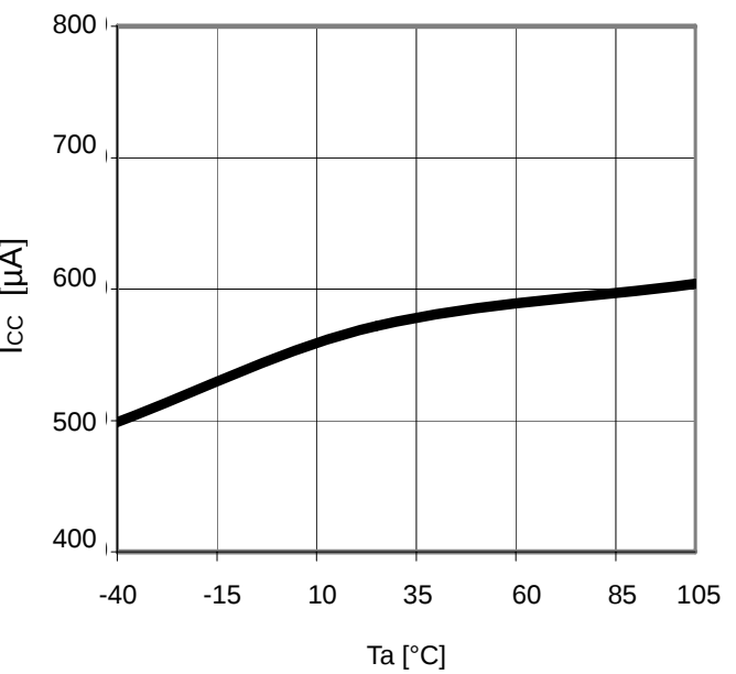
Fig.22 T_a - I_{cc}
