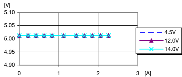
Output voltage vs. load current at T ref = +25°C
