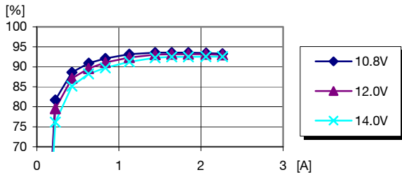
Efficiency vs. load current and input voltage at T ref = +25°C
