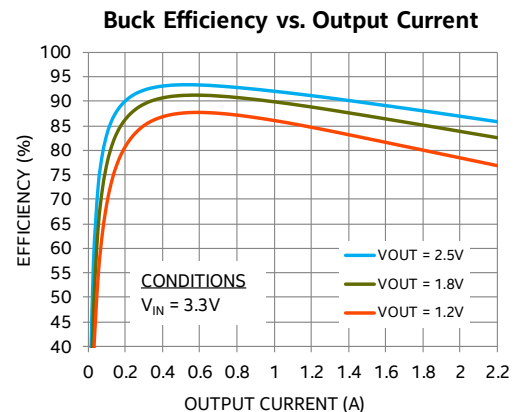
Figure 2: Efficiency at VIN = 3.3V
