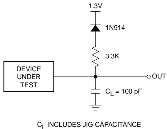
Figure 2. A.C. Testing Load Circuit (example)
