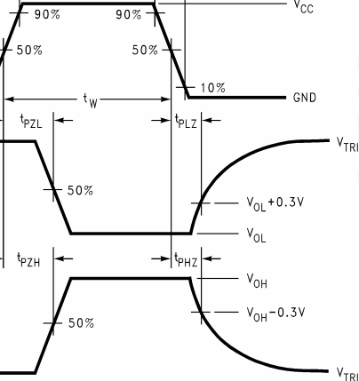
Figure 6. AC Waveforms
