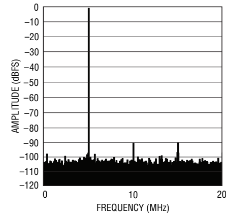
LTC2264-14: 8k Point FFT, f_{IN} = 5\text{MHz} , -1dBFS, 40Msps
