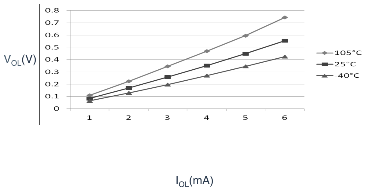
Figure 7. Typical I_{OL} Vs. V_{OL} (standard drive strength) ( V_{DD} = 3\text{ V} )
