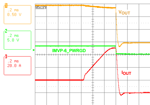
FIGURE 23. OVERCURRENT PROTECTION
